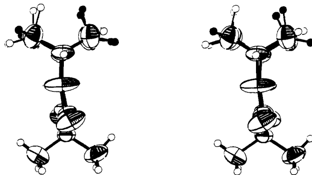
Figure 8. Stereoscopic view VIII.
