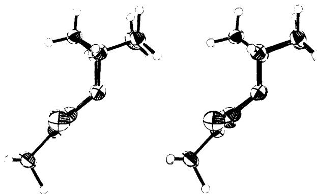
Figure 2. Stereoscopic view of II.
