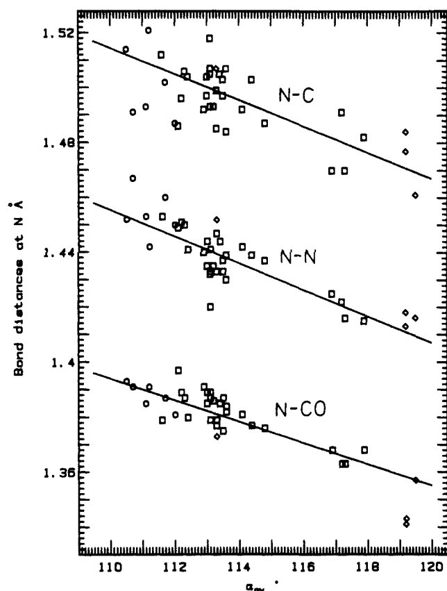
Figure 14. Variation of the bond lengths (Å) involving hydrazone nitrogen atoms, with the average bond angle around them ( \alpha_{av} ).
