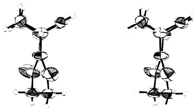
Figure 11. Stereoscopic view of XI.
